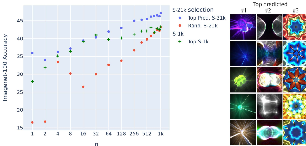
Figure 7: I-100 Top-1 accuracy with 100k images and SimCLR with different sets of shaders selected: 1) at random from Shaders-21k and 2) by predicted performance from all Shaders-21k that remain unseen while training the predictor. As a reference, we also plot the performance of the top shaders of Shaders-1k, but we note that this is a more limited set than the full Shaders-21k. The right-most columns are images from the top predicted shaders from Shaders-21k, the best best-performing one achieving 36% top-1 accuracy empirically, compared to 26% for the best in Shaders-1k.
