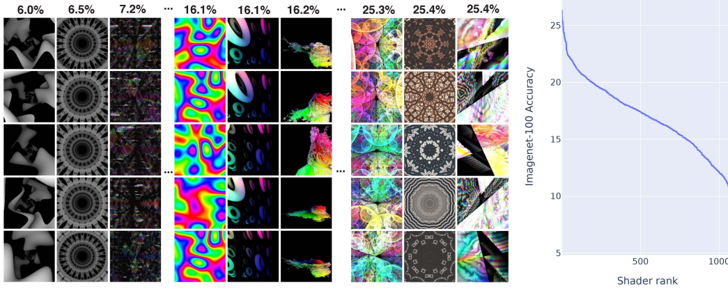
Figure 5: Left: Performance for the shaders in Shaders-1k trained with SimCLR on 10k images, evaluated on 10k samples of ImageNet-100. Left-to-right: images for different shaders sorted by performance (on top of each block). Right: I-100 accuracy of shaders in Shaders-1k, sorted by rank.
