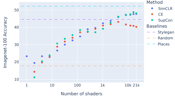
Figure 3: Linear classification performance on ImageNet-100 using a ResNet-18 trained with three representation learning methods and 100k images while varying the number of shaders. As dashed lines, we show performance with SimCLR trained on StyleGAN Oriented (state-of-the-art baseline), Places365 (upper bound), and a random network (lower bound).
