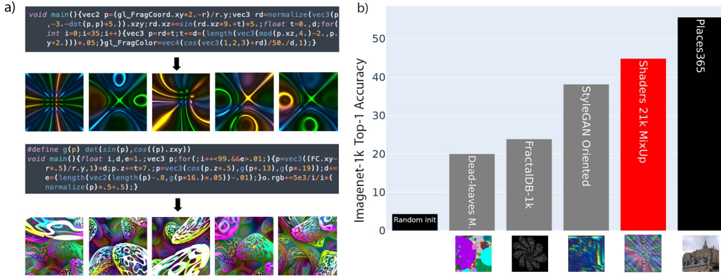
Figure 1: a) We propose learning image representations using a vast collection (21k) of short OpenGL fragment shaders. The code and rendered images for two of them are shown. b) Top-1 Accuracy on ImageNet-1k for linear classification with a ResNet-50 pre-trained with procedurally generated images from previous methods (Dead-Leaves Mixed [2], FractalDB [1] and StyleGAN Oriented [2], in gray) and our best generative image model, Shaders-21k with MixUp (in red). The lower and upper-bound performance (in black) is for a random initialization and pretraining with Places365 [6].
