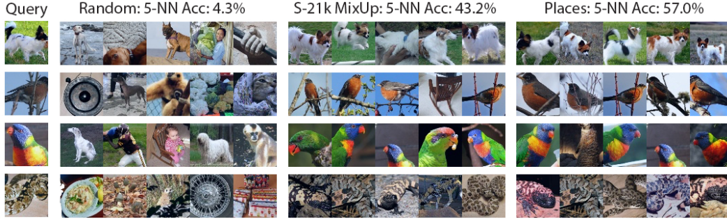
Figure 4: 5 nearest neighbors on ImageNet-100 for ResNet-50 randomly initialized (left) or trained with MoCo v2 on Shaders-21k with MixUp (middle) and Places365 (right). Reported accuracy corresponds to 5-NN accuracy on ImageNet-100.
