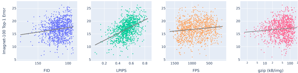
Figure 6: I-100 Performance against FID, LPIPS self-similarity, rendering time (frames per second), and gzip compression (for 400 images). Performance increases with lower FID (activations more similar to ImageNet images), lower self-similarity, higher rendering time (low FPS), and higher gzip file size, though the correlation is weak except for LPIPS self-similarity.
